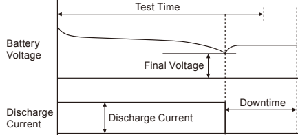
Transition of Constant current discharge → Voltage drop to final voltage → Discharge end → Discharge pause
