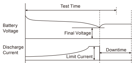
Transition of Constant power discharge → Voltage drop to final voltage → Discharge end → Discharge pause
