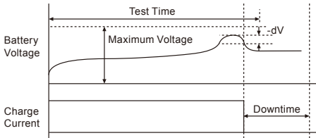
Transition of constant current charge → -dV detection → Charge end → Charge rest
