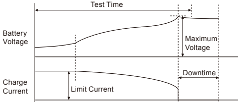
Transition of Limit current (CC) charge → Constant power charge → Maximum voltage detection → Charge end → Charge rest (Example of charge ending at maximum voltage)
