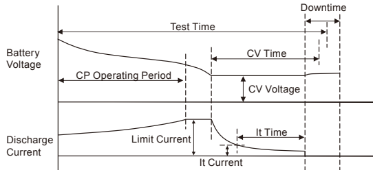
Transition of Constant power discharge → Constant voltage discharge → CV time reached → Charge pause (Example of discharging terminating at It time)
