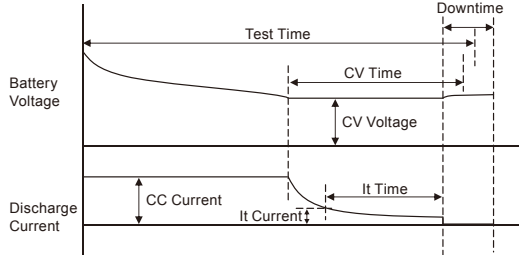
Transition of Constant current discharge → Constant voltage discharge → CV time reached → Charge pause (Example of discharging terminating at It time)
