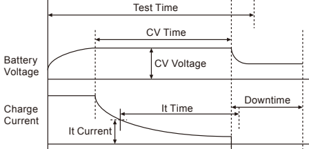
Transition of Constant current charge → Constant voltage charge → CV time reached → Charge pause (Example of charging terminating at CV time)
